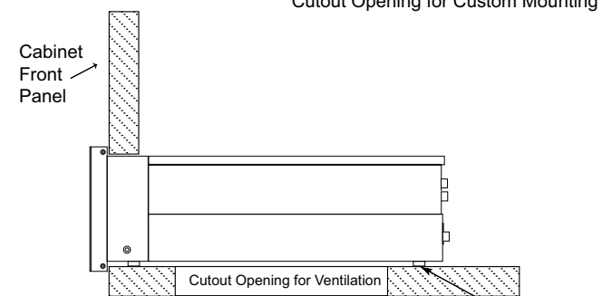
MCD350 Side View in Custom Cabinet
