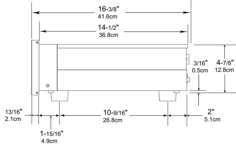
Side View of the MCD350
