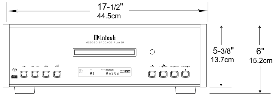
Front View of the MCD350
