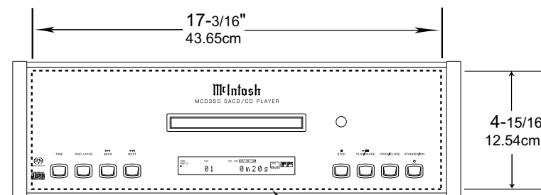
MCD350 Front Panel Custom Cabinet Cutout
